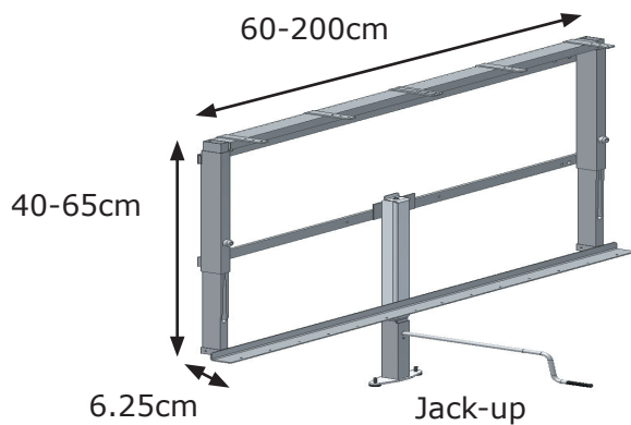
Frame for wall units Item 30-60060 - 30-60200
